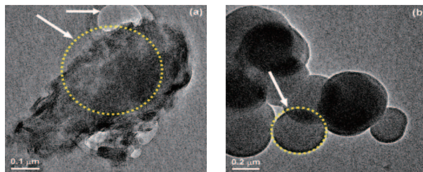
Figure 1. HR-TEM images of \text{TiO}_2\text{-SO}_4^{2-} : a) 100 nm ( \Rightarrow : corroded), b) 200 nm ( \Rightarrow : globular or round-shaped particle).
