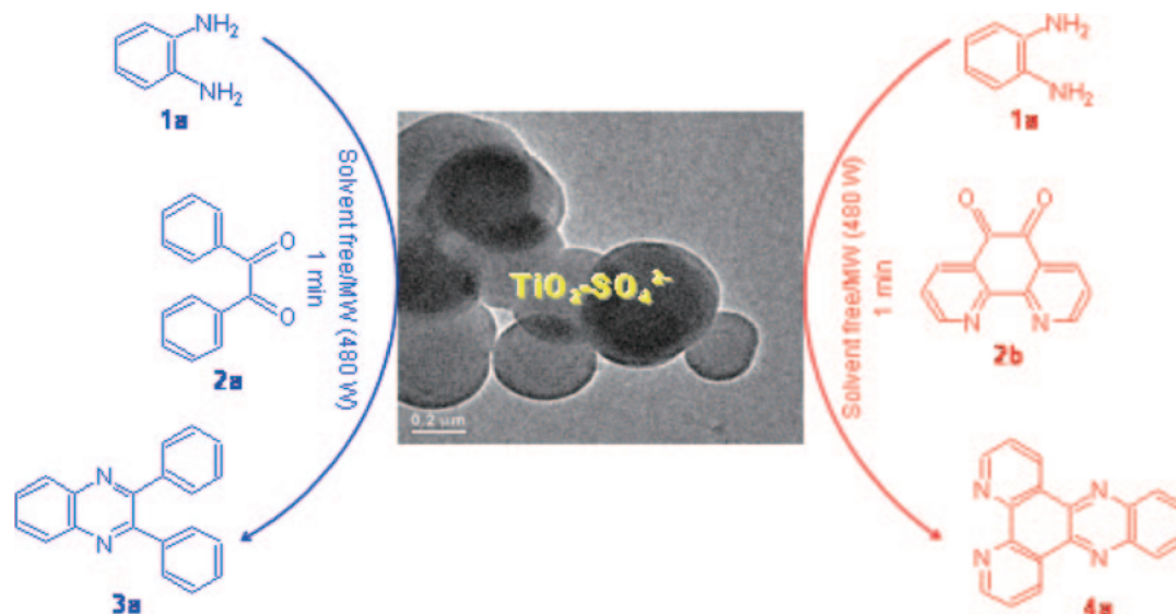
Scheme 1. The condensation reaction of o -phenylenediamine ( 1a ) with diketone (benzil ( 2a ) and 1,10-phenanthroline-5,6-dione ( 2b )) catalyzed by \text{TiO}_2\text{-SO}_4^{2-} under microwave irradiation.
