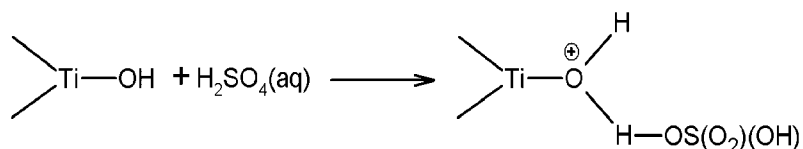
Scheme 2. Protonation of titania hydroxys by sulfuric acid.
