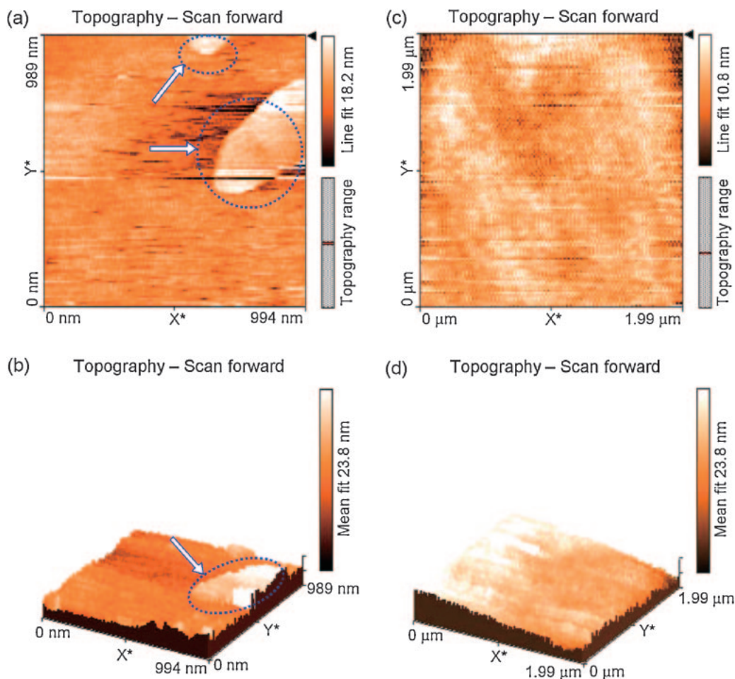
Figure 2. AFM images of a) \text{TiO}_2\text{-SO}_4^{2-} 2D image ( \Rightarrow : corroded), b) \text{TiO}_2\text{-SO}_4^{2-} 3D image ( \Rightarrow : corroded), c) prepared \text{TiO}_2 2D image, and d) prepared \text{TiO}_2 3D image.
